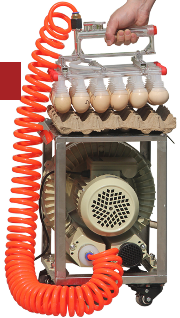
602 ZYS-ZK-30 Vacuum egg lifter
