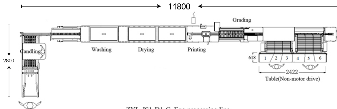
ZYL-JS1-D1-C Egg processing line Product code: 302AS Capacity: 10000 eggs/hour
